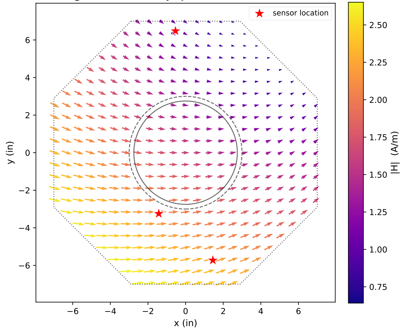
Magnetic Field Map ( J=66.04 A/in 2 , Pair P1)
